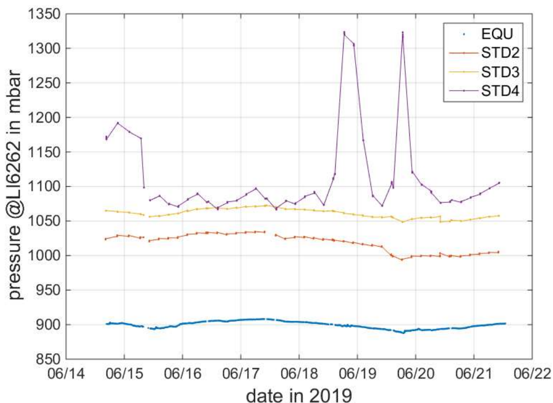
Figure 8: Pressure readings before the LI7815.
