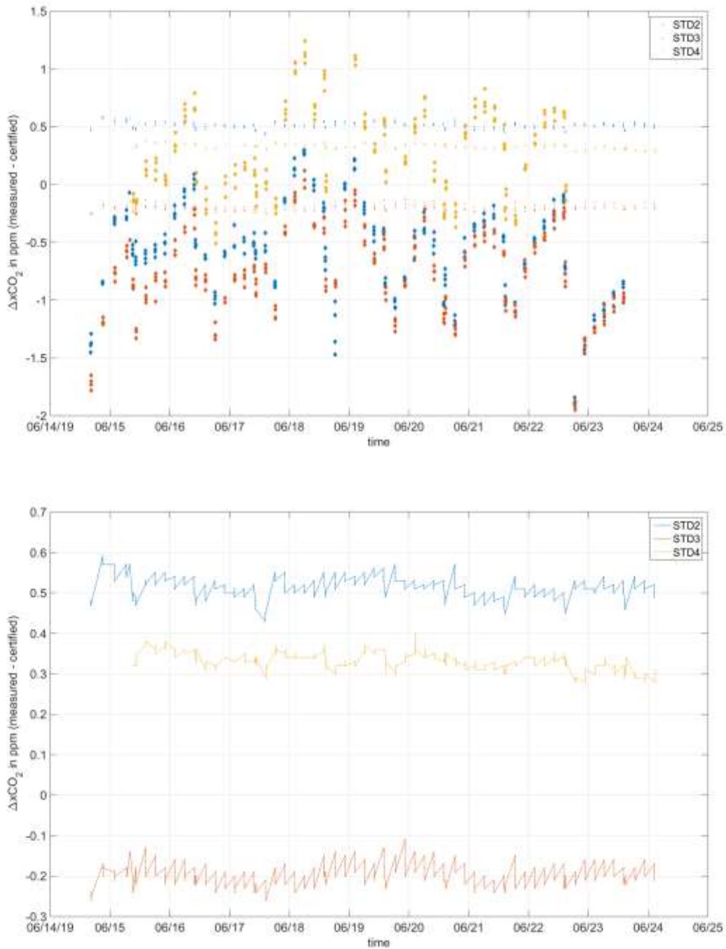
Figure 9: Data from standard gas measurements with the LI6262 (upper panel) and LI7815 (lower panel). The difference between the measured and the certified value for all three non-zero standard gases is shown. The standard deviation for measurements with the LI7815 is: \sigma(\text{STD2}) = 0.028 \text{ ppm} , \sigma(\text{STD3}) = 0.026 \text{ ppm} , \sigma(\text{STD4}) = 0.022 \text{ ppm} .
