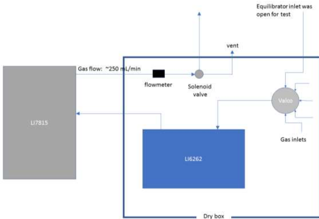
Figure 1: Schematic of connections for the LI7815 within the GO system in series with the LI6262. Please note that, for the beginning of our tests, the dry box was not connected to the wet box.
