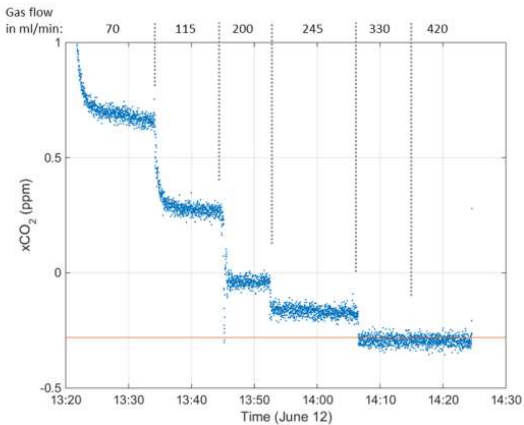
Figure 6: CO 2 readings of the LI7815 for different gas flows at the GO system. Both sensors (LI7815 and LI6262)9 were connected in parallel. The red line shows the approximate values for the zero standard measured before and after this test, when the sensors were connected in series.
