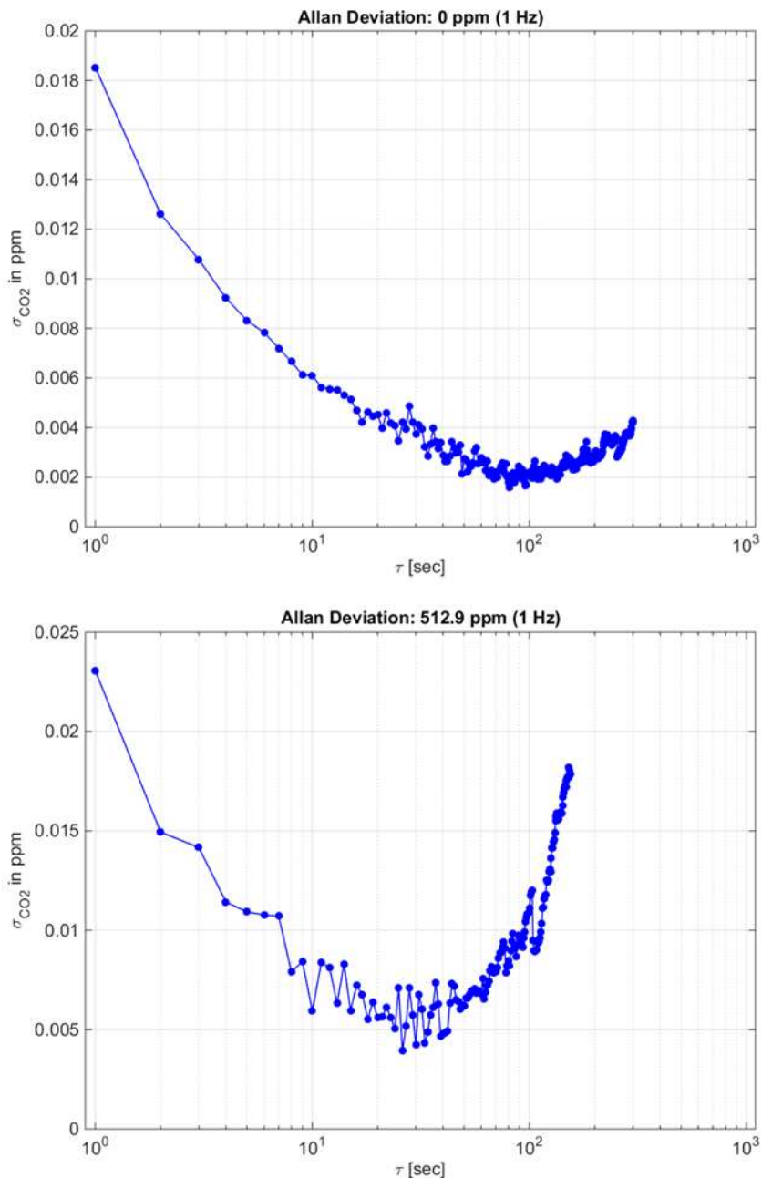
Figure 4: Allan deviation plots for CO 2 measurements at 1 Hz. The upper panel shows data for measuring the zero standard and the lower panel shows data from measuring the standard gas with 512.9 ppm CO 2 .
