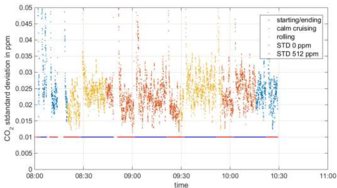
Figure 3: Standard deviation of CO 2 values averaged over 20 seconds during the rolling experiment onboard Littorina. The data are color coded for the periods where the ship was moving out of/into port and for the times where the ship was heavily rolling or calmly sailing. The color code of the line at 0.01 denotes the standard gas that was measured. The higher values above 0.035 ppm are from the period after the standard gas was changed, which typically leads to a higher standard deviation.
