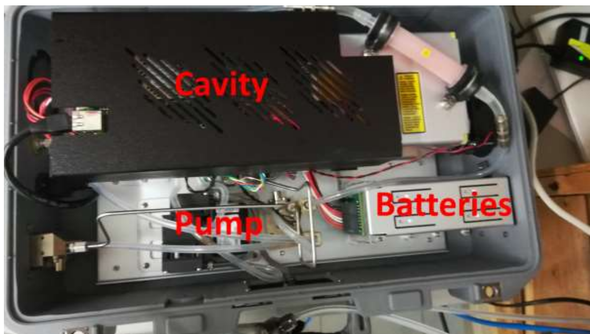
Figure 2: Inside view of LI7815. Each component can be removed separately.
